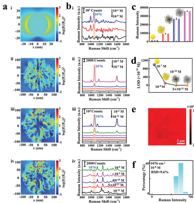
Fig. 4 Evaluation of SERS signal and electromagnetic field amplification for the proposed four different NPs. (a) FDTD simulation of the electric field distribution in the xz-plane for Au NP (i), spiky Au NP (ii), spiky Au@Ag NP (iii) and etched spiky Au@Ag NP (iv). (b) SERS spectra of 4-ATP on the Au NPs (i), spiky Au NPs (ii), spiky Au@Ag NPs (iii) and etched spiky Au@Ag NPs (iv) monolayer films. (c) Average Raman intensities at 1076 cm -1 peak of 4-ATP (10 -6 M) on the proposed four NPs monolayer films. (d) The limit of detection (LOD) of 4-ATP on the proposed four NPs monolayer films. (e) SERS intensity mapping images of 4-ATP (10 -6 M) measured at the 1076 cm -1 peak across a 10 × 10 μm 2 piece with 2 μm interval of the etched spiky Au@Ag NP monolayer films. (f) Histogram of Raman signal intensity at 1076 cm -1 of 4-ATP at the concentration of 10 -8 M on the etched spiky Au@Ag NP monolayer films.
