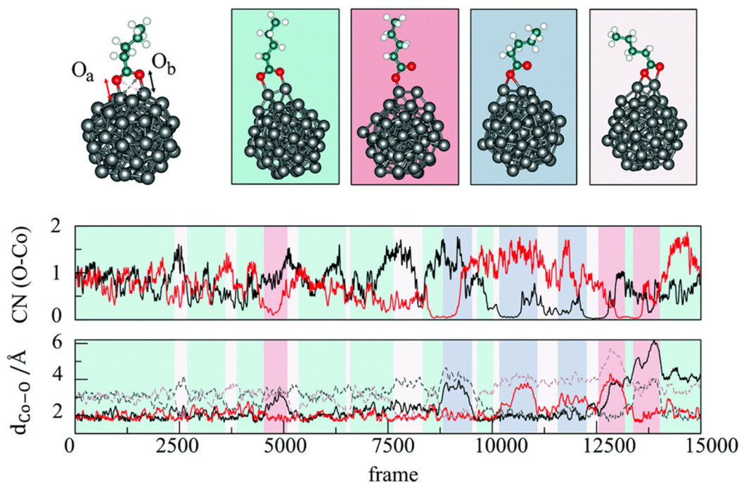
Fig. 27 Representative structures sampled during metadynamics simulations (top). Changes in the coordination numbers CN (middle), and Co–O bond distances d_{Co-O} (bottom) throughout the metadynamics trajectory. Reproduced from ref. 229 (copyright 2020, Royal Society of Chemistry).
