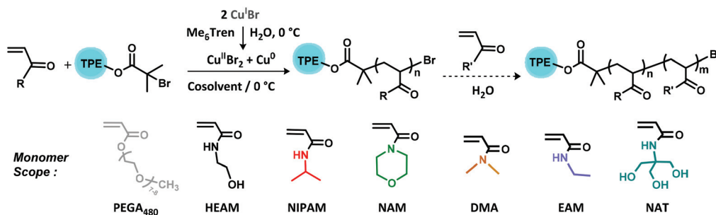
Scheme 1 Reaction scheme for homopolymerizations and in situ block copolymerizations of acrylamides and PEGA 480 with initiator TPEIB in aqueous Cu-RDRP at 0 °C.
