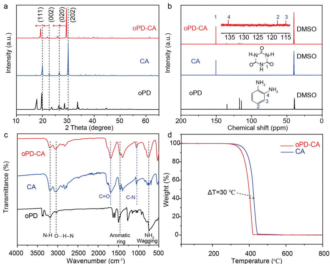
Fig. 1 (a) Powder XRD patterns, (b) 13 C-NMR spectra, (c) FTIR spectra of as-synthesized oPD-CA, pristine CA, and oPD, and (d) TG curves of oPD-CA, and the pristine CA in the nitrogen environment.
