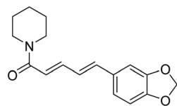
Piperine
