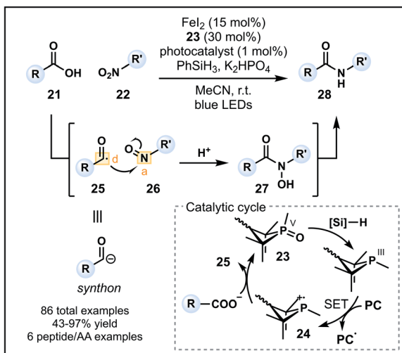
Fig. 4 Umpolung amidation utilizing the \text{P}^{\text{(III)}}/\text{P}^{\text{(V)}} catalytic cycle. Key intermediates that are important in umpolung C–N bond formation are shown. PC = photocatalyst; SET = single electron transfer; AA = amino acid.
