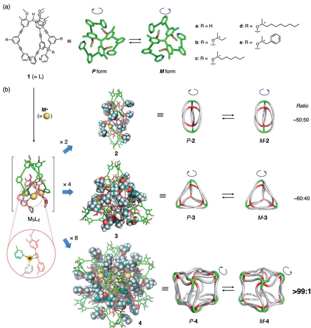
Fig. 1 (a) Chemical structure of propeller-shaped ligand 1 and its P - and M -forms. Unless otherwise noted, the ( S )-2-alkoxy isomers of 1b – e were used in the main study. (b) Schematic representation of the self-assembly of the (M_3L_2)_n coordination polyhedra 2 – 4 ( n = 2, 4, 8 ) with chiral side chains. Each assembly is formed by the oligomerization of n units of M_3L_2 , a hypothetical intermediate stabilized by metal–acetylene \pi -coordination. Illustrations in the second column from the left were generated by combining 2-butoxy side chains (molecular-mechanics (MM) models) with polyhedral frameworks based on the reported crystal structures. 8a,c Cartoon illustrations in the third column exhibit the entangled structures 11 of the (M_3L_2)_n polyhedra, while metal–acetylene \pi -coordination is omitted for clarity. 8c
