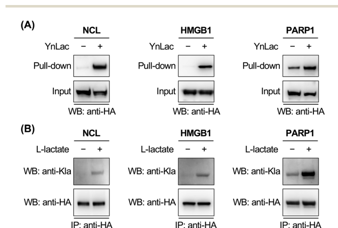
Fig. 4 Validation of the identification of selected lactylated non-histone proteins. (A) Verification of the enrichment of newly identified lactylated non-histone proteins. HEK293T cells expressing HA-tagged candidate lactylated proteins were labelled with YnLac (20 mM) for 8 hours and lysed for click conjugation with az-biotin. After pull-down with streptavidin beads, the enriched proteins were eluted for western blot analysis. (B) Verification of the lactylation of newly identified non-histone proteins. HEK293T cells expressing HA-tagged candidate lactylated proteins were treated with or without sodium L-lactate (25 mM) and lysed for immunoprecipitation. The immunoprecipitates were analyzed by western blot using a pan anti-lactyllysine antibody (anti-Kla). Anti-HA blotting shows the protein loading for each lane.
