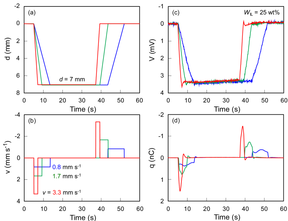
Fig. 6 Relation between input mechanical stimuli of (a) constant bending displacement ( d = 7 mm) with (b) different velocities ( v = 0.8, 1.7 , and 3.3 mm s ^{-1} ) and output electric signals of (c) voltage ( V ) and (d) electric charge ( q ) of ionic SMP gel sensor ( W_{IL} = 25 wt%).
