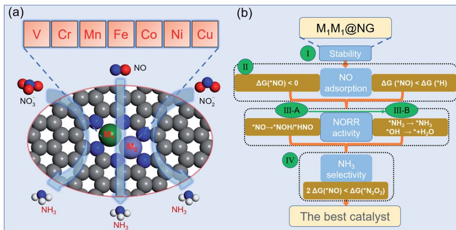
Fig. 1 (a) The atomic structure of M_1M_2@NG DACs ( M_1/M_2 = V, Cr, Mn, Fe, Co, Ni, Cu ). (b) The optimized strategy for screening NORR electrocatalysts including four stepwise selection principles. The third criterion consists of “two steps of key hydrogenation process”.
