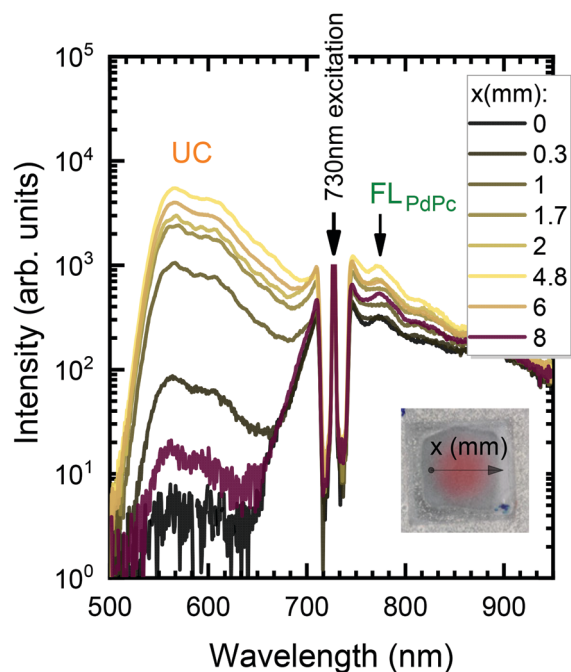
Fig. 6 Semi-log plot of UC emission spectra of PS: PdPc /Rub film measured at different excitation spots along x direction (indicated). Excitation, 730 nm. PdPc concentration in PS, 0.1 wt%. Sensitizer layer thickness, 110 nm. A picture of UC film is shown in the inset.
