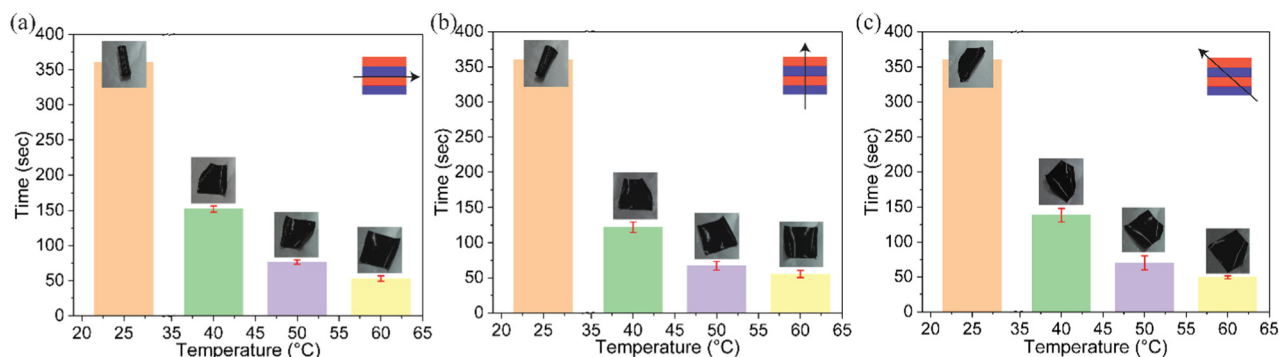
Fig. 2 Thermal-responsiveness demonstration study showed the response time as a function of temperature for 5L multiphase samples rolled (a) along with the layers (arrow direction in the insert figure), (b) perpendicular to the layers (arrow direction in the insert figure), and (c) diagonally at 45^\circ (arrow direction in the insert figure) with photographs showing the corresponding morphing stages.
