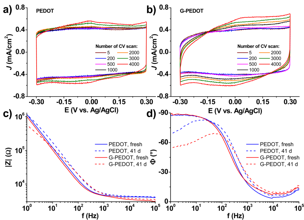
Fig. 4 Electrochemistry of PEDOT and G-PEDOT microelectrodes (50 × 50 μm) prepared by galvanostatic electropolymerization (2 μC: 20 nA, 100 s) (a and b): selected cyclic voltammograms (scan rate = 100 mV s -1 ) over 4000 cycles (electrochemical stability test); (c and d): electrochemical impedance spectra (bode plots, averaged over 2–3 different specimens) as prepared and after 41 days of accelerated aging test (60 °C, PBS solution).
