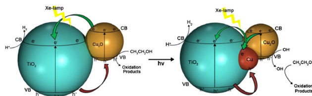
Fig. 17 H 2 -Production mechanism from photoreforming of ethanol using Cu 2 O/Cu/TiO 2 under Xe-lamp irradiation. Reprinted with permission from Elsevier. 212,214
