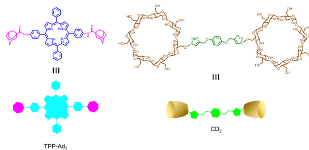
Fig. 14 Chemical structures of the adamantyl-modified tetraphenyl porphyrin (TPP-Ad 2 ) and the cyclodextrin dimer (CD 2 ).
