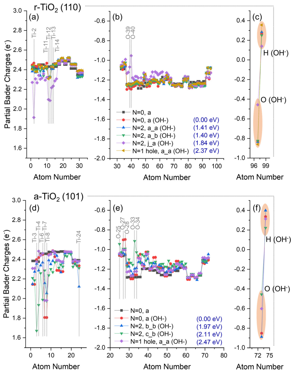
Fig. 6 Partial Bader charges over (a–c) OH - /r-TiO 2 (110) and (d–f) OH - /a-TiO 2 (101) surfaces when considering the ground state ( N = 0 , a; and N = 0 , a (OH - )) of the electronic structure, as well as triplet state ( N = 2 b_b (OH - ) and N = 2 c_b (OH - )) and hole-containing electronic structure ( N = 1 hole, a, (OH - )). Charges of respective clean surfaces are given for comparison. Charges over Ti ions (a and d), O ions (b and e), and adsorbate (c–f) are individually presented. The relative energy ( E_{\text{rel}} ) of each structure is given in parentheses. Atom numbers refer to labels defined in the methodology section.
