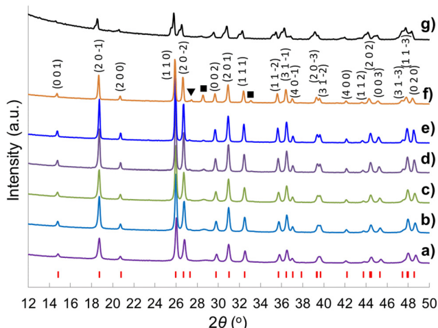
Fig. 1 XRD patterns of (CeTi 2.05 )O 6 -complex powders calcined for 6 h at (a) 600 °C, (b) 700 °C, (c) 800 °C, (d) 900 °C, (e) 1050 °C, (f) 1150 °C, (g) 1250 °C. The red vertical markers beneath the brannerite patterns show the peak positions expected in the crystal structure. (▼) rutile-type TiO 2 , (■) CeO 2 .
