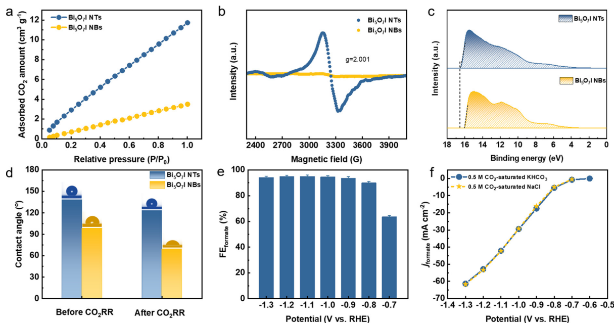
Fig. 6 (a) CO 2 adsorption isotherms, (b) EPR spectra, (c) UPS spectra and (d) contact angle measurements before and after the CO 2 RR on Bi 5 O 7 I NTs and NBs, (e) FE formate and (f) J formate of Bi 5 O 7 I NTs in CO 2 -saturated 0.5 M NaCl.
