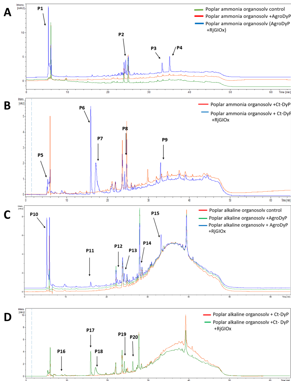
Fig. 6 Total ion chromatograms for product formation from combined DyP/GiOx transformations of polymeric lignin substrates. Bioconversion of poplar ammonia organosolv lignin by AgroDyp/RjGiOx (A) and CtDyp/RjGiOx (B), and conversion of poplar alkaline organosolv lignin by AgroDyp/RjGiOx (C) and CtDyp/RjGiOx (D), are compared with control incubations containing DyP peroxidase alone, or no enzyme. Peaks that show increased intensity or are absent without RjGiOx are indicated, and they are identified in Table 2.
