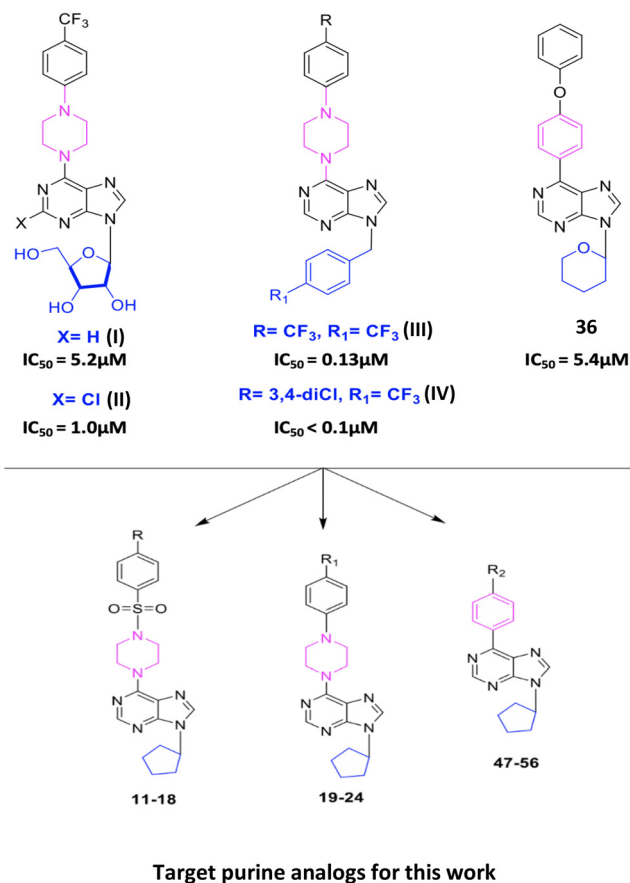
Fig. 1 Structures of 9-(β-D-ribofuranosyl)/4-trifluoromethyl/4-chlorobenzyl/tetrahydropyran)-6-(4-trifluoromethylphenylpiperazine/4-phenoxyphenyl) purine analogs (I), (II), (III), (IV), and 36 and target purine compounds 11–24 and 47–56.
