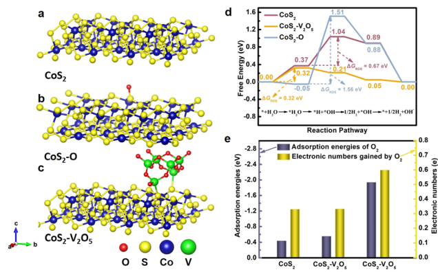
Fig. 5 (a–c) Crystal structures of CoS 2 , CoS 2 -O and CoS 2 -V 2 O 5 , (d) comparison of standard Gibbs free energies at the rate determining step of CoS 2 , CoS 2 -O and CoS 2 -V 2 O 5 during the HER process, and (e) the adsorption energies of O 2 molecules at metal sites (Co sites and V sites) and the electronic numbers gained by O 2 molecules.
