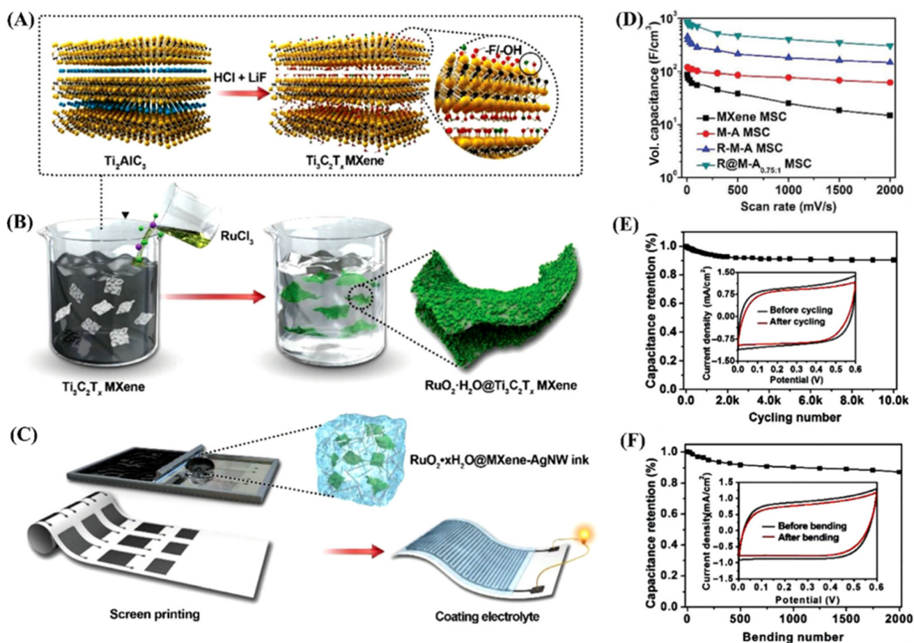
Fig. 7 Illustration of (a) the preparation of Ti 3 C 2 T x MXenes; (b) procedure for the synthesis of the RuO 2 · x H 2 O@MXene nanocomposite; (c) development of flexible MSC devices through screen printing; a graphical image showing (d) the volumetric capacitance of various MXene MSCs at diverse scan rates; (e) plot of cycling stability at 100 mV s -1 (inset: CV curves recorded before and after cycling); and (f) plot of cycling stability with a bending strain of 5.0% at various bending cycles (the inset shows CV curves recorded before and after 2000 bending cycles at 100 mV s -1 ). 108 Reproduced from ref. 108 with permission from Wiley-VCH, copyright 2019.
