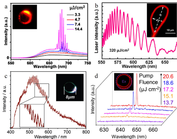
Fig. 7 Laser performance from ring resonators of organic micro/nano-crystals. (a) The PL spectra of CAZ-A/CBP microrings at different pump energies with a diameter of 19 \mu\text{m} . Inset: the PL microscopy image of this corresponding microring excited above the laser threshold. 47 Copyright 2019, American Chemical Society. (b) The PL spectrum of QD doped PVP ring nanowire pumped with the density 320 \mu\text{J cm}^{-2} . Inset: PL microscopy image of an individual ring with D is 26 \mu\text{m} and d is 11 \mu\text{m} . 16 Copyright 2014, American Chemical Society. (c) The PL spectrum of single DPPDO microring with a diameter of 8 \mu\text{m} . The excitation position is marked with a violet circle. Inset is the PL microscopy image of the corresponding microring pumped with the focused 351 nm laser. 37 Copyright 2013 Wiley-VCH Verlag GmbH & Co. KGaA, Weinheim. (d) The PL spectra of the HDFMAC double-microring as a function of pump density. Inset is the PL microscopy image of a coupled ring resonator. 43 Copyright 2019, American Chemical Society.
