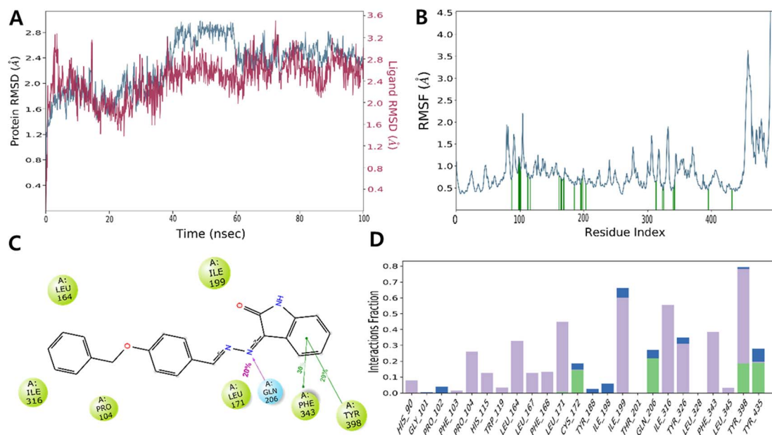
Fig. 8 Molecular docking (MD) simulation analysis of ISB1-MAO-B complex. Root-mean-square deviation (RMSD) (A) and root-mean-square fluctuation (RMSF) of various amino acids (B). A 2D interaction diagram of ISB1-MAO-B complex (C). Protein–ligand contact analysis of the MD trajectory (D). In panel (A), the RMSD of protein and ISB1 are depicted in blue and red, respectively.
