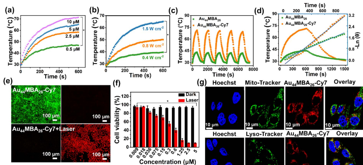
Fig. 2 In vitro PTT of the Au 44 MBA 26 -Cy7 NCs. Photothermal heating profiles of the Au 44 MBA 26 -Cy7 NCs in water at (a) different concentrations under laser irradiation (808 nm, 1.5 W cm -2 ) and (b) different power density irradiations (here the NC concentration was fixed to 5 μM). Error bars, mean ± SD ( n = 3), * P < 0.05. (c) The cycled heating/cooling curves of pristine Au 44 MBA 26 and Au 44 MBA 26 -Cy7 NCs in water. (d) Photothermal efficiency evaluation of the Au 44 MBA 26 and Au 44 MBA 26 -Cy7 NCs in water after irradiation for 10 min and being cooled to room temperature. The photothermal efficiency was obtained from the linear fitting of the cooling time versus the negative natural logarithm of the temperature. (e) PL microscope images of viable HeLa cells stained with Calcein AM (green color) and nonviable HeLa cells stained with EthD-1 (red) treated with 5 μM Au 44 MBA 26 -Cy7 NCs in the dark (upper panel) or under laser irradiation (lower panel) for 6 min (808 nm, 1.5 W cm -2 ). (f) In vitro cytotoxicity and photothermal assays of Au 44 MBA 26 -Cy7 NCs with different concentrations (0.009–5 μM) on HeLa cells evaluated by MTT Kit NCs in the dark or under laser irradiation. Error bars indicate the mean ± SD ( n = 8), * P < 0.05. (g) Confocal PL images of Au 44 MBA 26 -Cy7 NCs (0.5 μM) in live HeLa cells co-stained with MitoTracker Green or LysoTracker Green.
