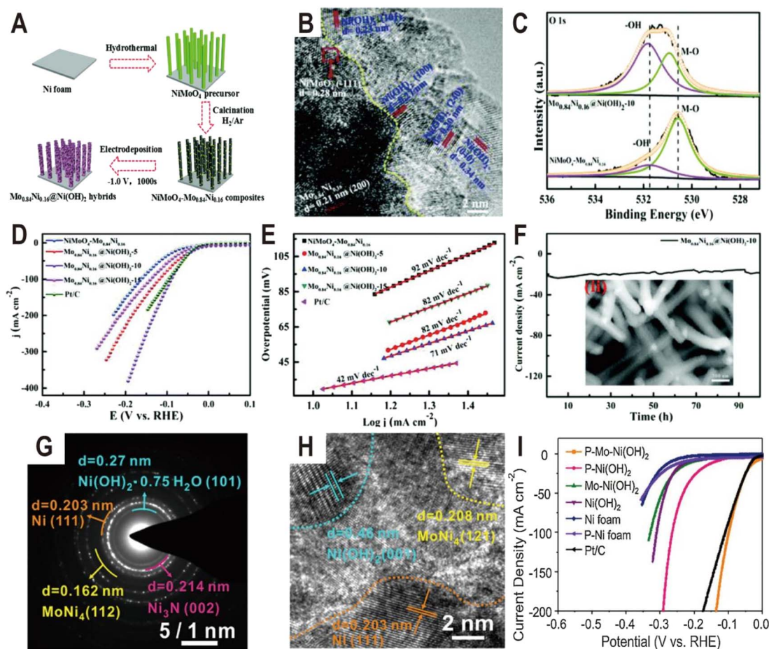
Fig. 6 (A) Schematic illustration of the preparation of the \text{Mo}_{0.84}\text{Ni}_{0.16}@Ni(\text{OH})_2 heterostructure. (B) HRTEM image of \text{Mo}_{0.84}\text{Ni}_{0.16}@Ni(\text{OH})_2 . (C) The high-resolution XPS spectra of O 1s for \text{NiMoO}_4-\text{Mo}_{0.84}\text{Ni}_{0.16} composites and the \text{Mo}_{0.84}\text{Ni}_{0.16}@Ni(\text{OH})_2 heterostructure. (D and E) Polarization curves and the corresponding Tafel plots of \text{NiMoO}_4-\text{Mo}_{0.84}\text{Ni}_{0.16} and \text{Mo}_{0.84}\text{Ni}_{0.16}@Ni(\text{OH})_2 with different deposition times of 5, 10, and 15 min, and Pt/C. (F) The chronoamperometric curve at an overpotential of 34\text{ mV} for \text{Mo}_{0.84}\text{Ni}_{0.16}@Ni(\text{OH})_2 . The inset is the SEM image after the stability test. Reproduced with permission. 59 Copyright 2020, Royal Society of Chemistry. (G and H) SAED pattern and HRTEM image of P-Mo-Ni( \text{OH})_2 NSAs. (I) Polarization curves of Ni foam, P-Ni foam, \text{Ni}(\text{OH})_2 NSAs, \text{Mo-Ni}(\text{OH})_2 NSAs, P-Ni( \text{OH})_2 NSAs, P-Mo-Ni( \text{OH})_2 NSAs, and Pt/C. Reproduced with permission. 60 Copyright 2020, Elsevier.
