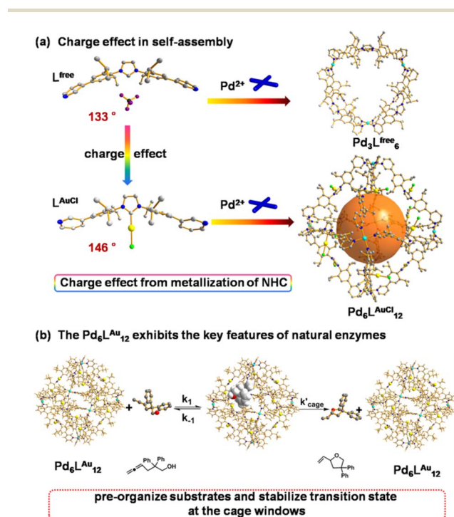
Fig. 1 (a) Charge effect of rigid NHC metallization-triggered supramolecular configurations. (b) The Pd 6 L Au 12 cage presents the features of enzymatic catalysis at the cage window for gold-catalyzed cyclization of allenol. The structures of L free , L AuCl and Pd 6 L AuCl 12 are their single crystal X-ray structures. The structure of Pd 3 L free 6 is a modelled structure. Color coding: C: gray; N: dark blue; Au: yellow; Pd: light blue; Cl: bright green; B: dark green; F: violet; O: red; H: white.
