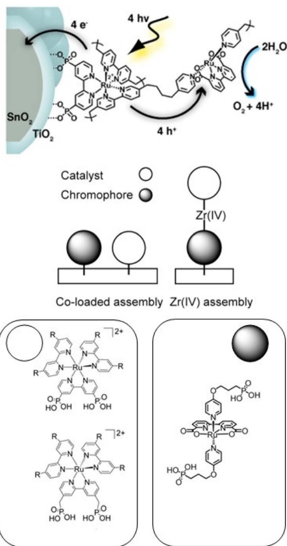
Fig. 8 Top: Covalent approach to anchor the Ru trisbipyridine photo-sensitizer and Ru(bda) WOC. Reprinted from ref. 89 with permission from the American Chemical Society, copyright 2015. Bottom: Co-loaded and Zr(IV) assembly approaches. Adapted from ref. 90 with permission from the American Chemical Society, copyright 2016.
