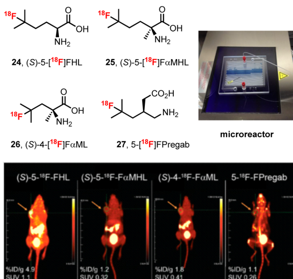
b) Dynamic PET imaging of (S)-5-[ 18 F]FHL (24)
