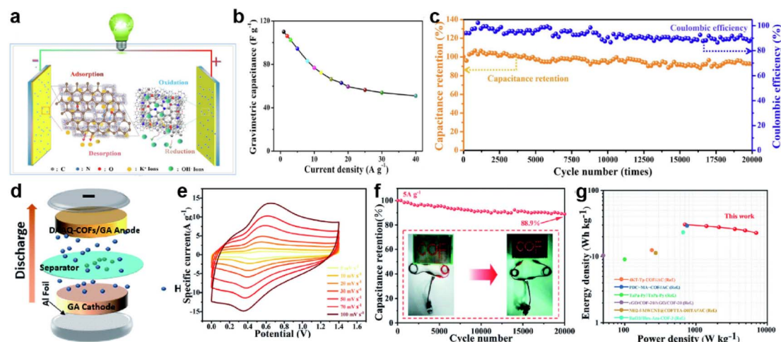
Fig. 15 (a) Schematic structure, (b) specific capacitance, and (c) cycling stability and coulombic efficiency of COF-900-based SSCs. Reprinted from ref. 125. Copyright 2023, Elsevier. (d) Schematic of the DAAQ-COFs/GA//GA ASC device. (e) CV curves of the ASC at different scan rates. (f) Stability test at 5 A g -1 for 20 000 cycles (the inset shows a digital photograph of the LED powered by the ASC). (g) Ragone plot of the ASC. Reprinted from ref. 102. Copyright 2021, Royal Society of Chemistry.
