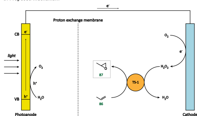
Fig. 13 Cathode-mediated in situ \text{H}_2\text{O}_2 generation for propylene epoxidation.
