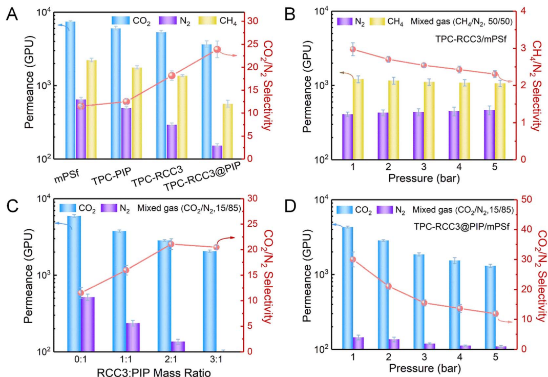
Fig. 4 (A) Pure \text{CO}_2 , \text{N}_2 , \text{CH}_4 permeances, and ideal \text{CO}_2/\text{N}_2 selectivity of the mPSf substrate and composite membranes fabricated with various reactive monomers. (B) Mixed \text{CH}_4/\text{N}_2 separation performance of the TPC-RCC3/mPSf composite membrane at different feed gas pressures. (C) Mixed \text{CO}_2/\text{N}_2 separation performance of the TPC-RCC3@PIP/mPSf ( x:1 , x = 0, 1, 2, 3 ) composite membranes at 2 bar. (D) Mixed \text{CO}_2/\text{N}_2 separation performance of the TPC-RCC3@PIP/mPSf composite membrane at different feed gas pressures.
