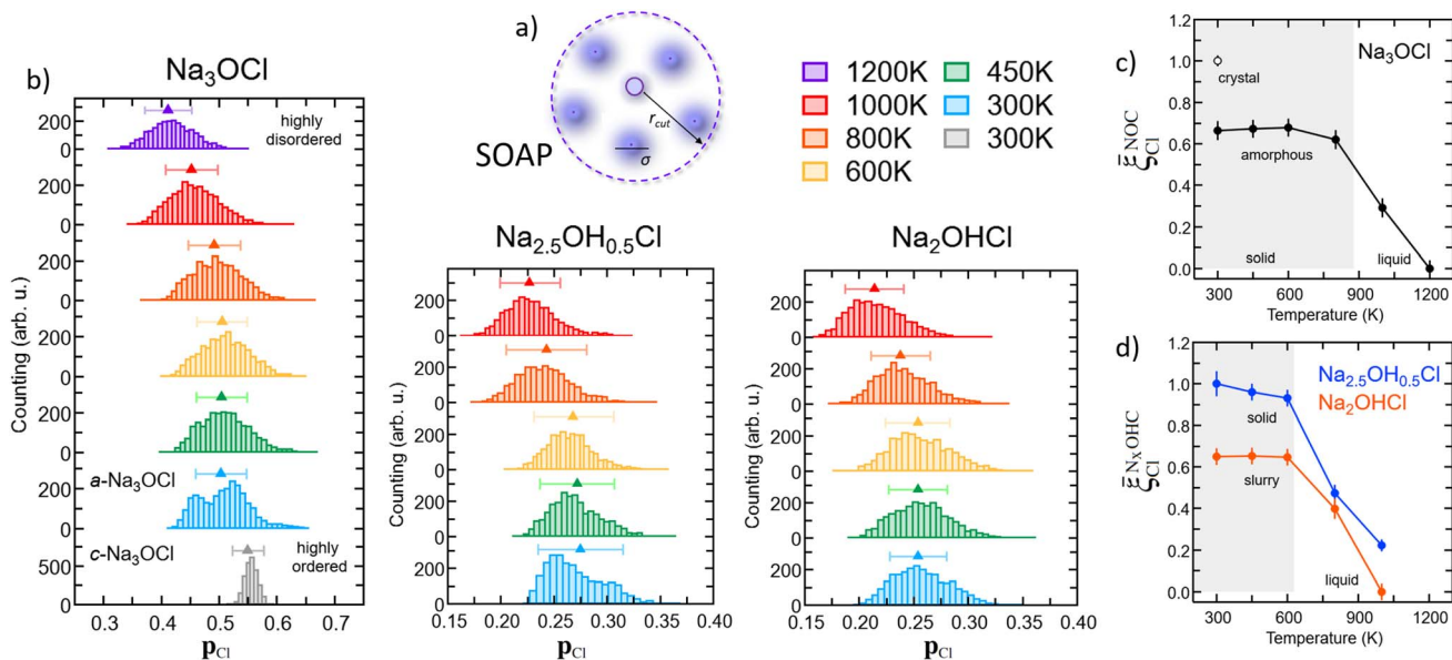
Fig. 7 (Color online) (a) Schematic representation of the SOAP descriptor. (b) Na_3OCl , Na_{2.5}OH_{0.5}Cl , and Na_2OHCl SOAP p_{Cl} distributions computed at different temperatures. The data computed for crystalline Na_3OCl are also reported. Structural disorder degree of the three models framed as SOAP similarity to crystalline Na_3OCl ( \xi_{Cl}^{NOC} , (c)) and to the amorphous Na_{2.5}OH_{0.5}Cl phase, ( \xi_{Cl}^{N_{x}OHC} , (d)), respectively.
