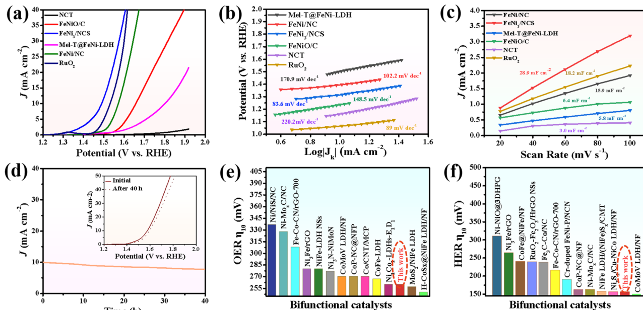
Fig. 3 (a) OER LSV profiles, (b) Tafel slopes, and (c) C_{dl} of \text{FeNi}_3/\text{NCS} , NCT, \text{FeNiO}/\text{C} , \text{FeNi}/\text{NC} , \text{Mel-T@FeNi-LDH} and \text{RuO}_2 . (d) Amperometric i-t of \text{FeNi}_3/\text{NCS} at 10 \text{ mA cm}^{-2} (inset: the polarization curve of \text{FeNi}_3/\text{NCS} after i-t measurement); comparison of (e) OER and (f) HER overpotential of this work and reported FeNi-containing electrocatalysts.
