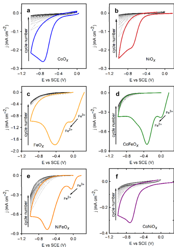
Fig. 3 Cyclic voltammograms at 20 mV s -1 of the deposition of the single (Ni, Co, Fe) and mixed (CoFe, NiFe, CoNi) metal oxides over 20 cycles. Potential regions for the electrochemical reactions discussed are noted. The cycle number increases from each initial cycle highlighted, to the subsequent cycles trending towards 0 current. (a) Co. (b) Ni. (c) Fe. (d) CoFe. (e) NiFe. (f) CoNi.
