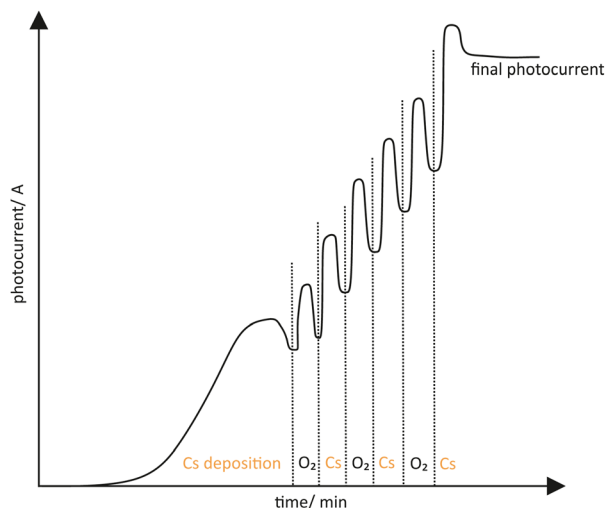
Fig. 9 Schematic drawing of a typical photocurrent evolution when a YoYo activation is used (alternately applying Cs and \text{O}_2 ).
