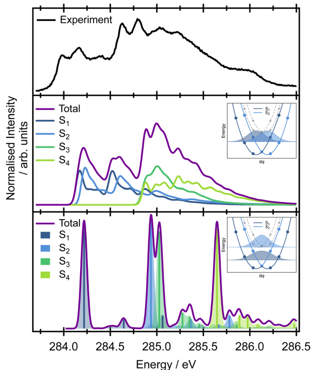
Fig. 3 Top panel: The pre-edge region of the C K-edge XAS spectrum of butadiene. Middle panel: Theoretical core XAS vibronic spectrum calculated at the SRC1-r1/cc-pCVTZ level with a vertical Franck-Condon approximation on a displaced Franck-Condon point geometry. Inset is a schematic of the lowest vibrational energy level of S_1 and S_2 for mode \nu_{21} to show the harmonic approximation (yielding diabatic states). Bottom panel: Calculated overlaps between the ground and excited state wave functions without the harmonic approximation (fully adiabatic framework). Inset is a schematic without the harmonic approximation. The energy splitting between the ground vibronic states is 0.38 eV in the exact case (note that it is exactly 0 eV in the harmonic approximation).
