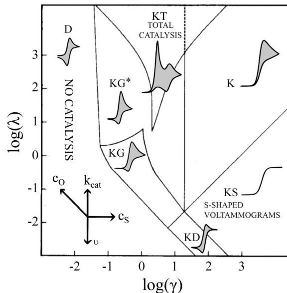
Fig. 6 Diagram of the catalytic zones for simulated CVs of one electron reduction of substrate S via a redox mediator, O. The kinetic parameter \lambda = \left(\frac{RT}{F}\right)\left(\frac{k_{\text{Cat}}c_O}{v}\right) and the excess factor \gamma = \frac{c_S}{c_O} represent the competition between catalytic rate and scan rate, and the initial electrolyte composition, respectively. The CV waveforms follow the convention of negative potentials to the right and cathodic current upward. Scans are started from positive potentials. Reprinted with permission from ref. 39. Copyright 2014 American Chemical Society.
