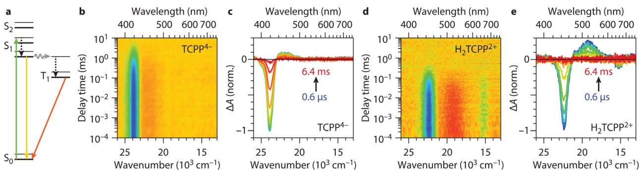
Fig. 2 Excited state dynamics of TCPP 4- and \text{H}_2\text{TCPP}^{2+} . (a) Jablonski diagram for TCPP neutral environment (region I), showing the excitation into the singlet (green arrow), vibrational relaxation (black arrow), singlet relaxation (yellow arrow), intersystem crossing (grey arrow), and triplet relaxation (orange arrow) pathways. The same applies to \text{H}_2\text{TCPP}^{2+} , i.e. fully protonated TCPP (region III), except that it does not have a split S_1 level (see text). (b) and (d) Transient absorption heatmaps on TCPP 4- and \text{H}_2\text{TCPP}^{2+} after excitation at respectively 515 nm and 665 nm. (c) and (e) Spectral slices of the heatmap at delay times 0.6 \mu\text{s} , 3.0 \mu\text{s} , 9.1 \mu\text{s} , 24 \mu\text{s} , 63 \mu\text{s} , 160 \mu\text{s} , 0.4 ms, 1.0 ms, 2.5 ms, and 6.4 ms from blue to red. The bleach positions correspond to the Soret bands in the steady state spectra (Fig. 1(b)). When fitting a single exponential to the bleach intensity time traces, lifetimes of 1.2 ms and 120 \mu\text{s} are obtained for TCPP 4- and \text{H}_2\text{TCPP}^{2+} respectively.
