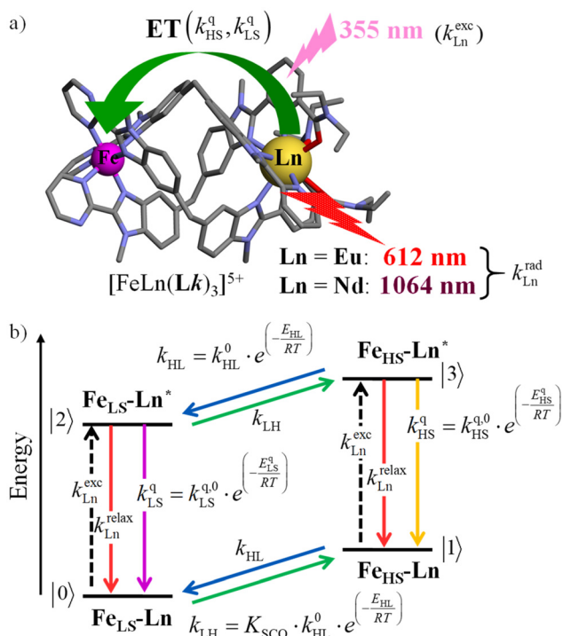
Fig. 8 (a) Fe(II)-modulated light downshifting operating in [\text{Fe(II)Ln(Lk)}_3]^{5+} helicates (ET = energy transfer) and (b) associated four-states kinetic model.
