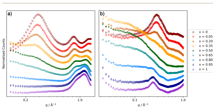
Fig. 5 (a) SAXS data and (b) SANS data collected for [C_{10}MIM]_{1-x}[C_{10}MIM-F_{17}]_x[Tf_2N] mixtures at 60 \text{ }^\circ\text{C} . Data for each composition are shifted along the y -axis for clarity. Note the different scales used for the x -axes.
