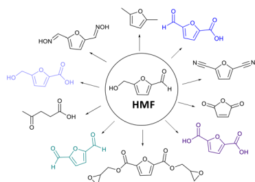
Fig. 1 HMF and value-added oxidized derivatives. 2,5-diformylfuran (DFF), 5-hydroxymethyl-2-furancarboxylic acid (HMFCFA), 5-formyl-2-furancarboxylic acid (FFCA), 2,5-furandicarboxylic acid (FDCA) and 5-hydroxymethylfurfural (HMF).
