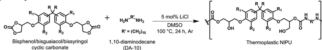
Scheme 1 Synthesis of (a) BGF/BSF using guaiacol/syringol and vanillyl/syringyl alcohol, (b) BGA/BSA using guaiacol/syringol and acetone, (c) diglycidyl ether of bisguaiacol/bissyringol from respective bisguaiacol/bissyringol and epichlorohydrin, (d) bisguaiacol/bissyringol cyclic carbonate from respective diglycidyl ether and CO 2 , and (e) NIPU using respective bisguaiacol/bissyringol cyclic carbonate and 1,10-diaminodecane (DA-10).
