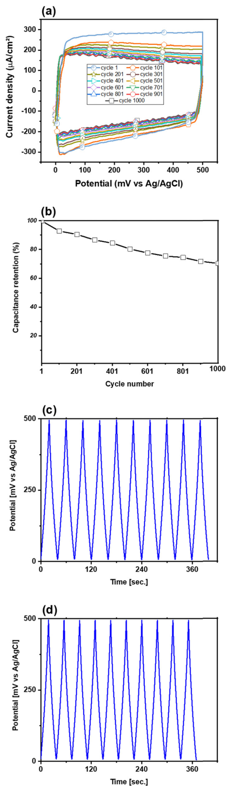
Fig. 7 (a) CV curves at a scan rate of 80 mV s -1 (1000 cycle number), (b) areal capacitance retention, (c) charge-discharge curve in the first 10 cycles and (d) charge-discharge curve in the last 10 cycles during 1000 cycles.
