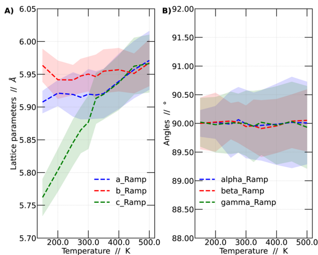
Fig. 2 (A) Variation of the average lattice parameters ( a , b and c ) and (B) angles among lattice vectors ( \alpha , \beta and \gamma ) as a function of temperature for \text{CsPbBr}_3 . The standard deviation (STD) is depicted using a shaded region.
