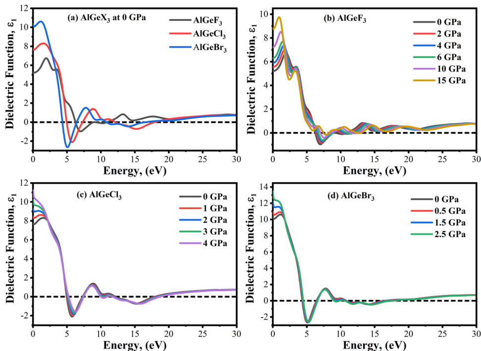
Fig. 6 Comparison of the real part of the dielectric constant without pressure (a) AlGeX 3 (X = F, Cl, and Br) and with pressure (b) AlGeF 3 , (c) AlGeCl 3 , and (d) AlGeBr 3 .
