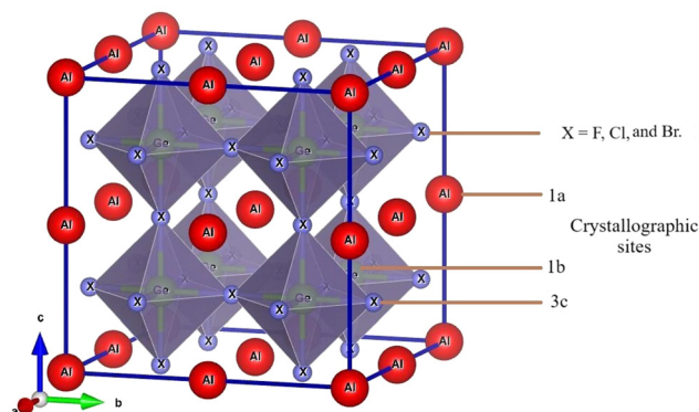
Fig. 1 \text{AlGeX}_3 ( X = \text{F, Cl, and Br} ) cubic metal halide perovskite structure.
