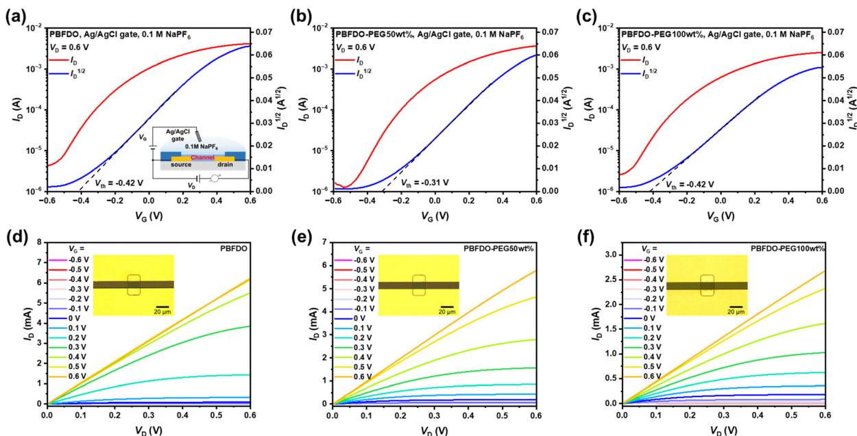
Fig. 4 Transfer (a)–(c) and output characteristics (d)–(f) of OECTs based on (a) and (d) PBFDO; (b) and (e) PBFDO-PEG50wt%; (c) and (f) PBFDO-PEG100wt%. The transfer characteristics were measured at V_{ds} = 0.6 V. The channel dimension used for this measurement is channel width/length = 20 \mu\text{m}/10 \mu\text{m} , while the thickness was around 70 nm. Inset: Illustration of the OECT structure (a) and optical microscopic photos of the corresponding OECT channels (d)–(f).
