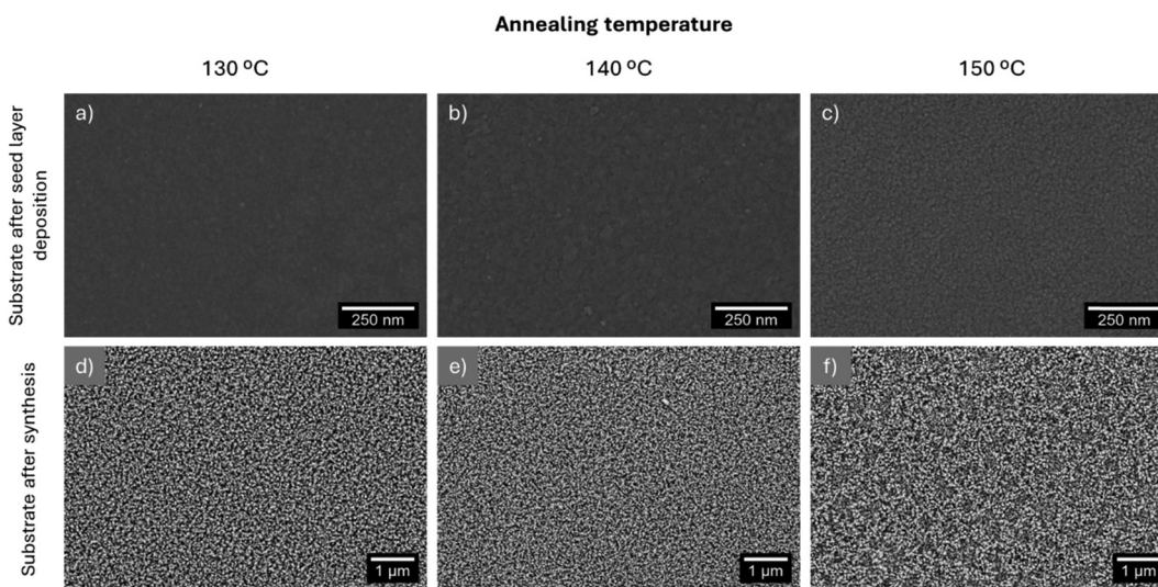
Fig. 2 Morphology of the flexographic printed seed layer and the ZnO nanorods grown from layers annealed at 130 (a) and (d), 140 (b) and (e) and 150 °C (c) and (f).
