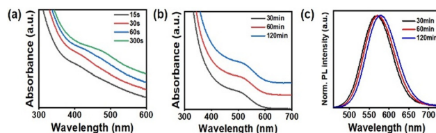
Fig. 2 (a) Temporal evolution of the UV-vis absorption spectra of the \text{In}(\text{Zn})\text{P} seed-mediated \text{Zn}_3\text{P}_2 QD growth solution during annealing at 270 °C up to 5 min. (b) UV-vis absorption spectra and (c) corresponding PL spectra of aliquots taken from the growth solution at 270 °C over extended periods up to 120 min.
