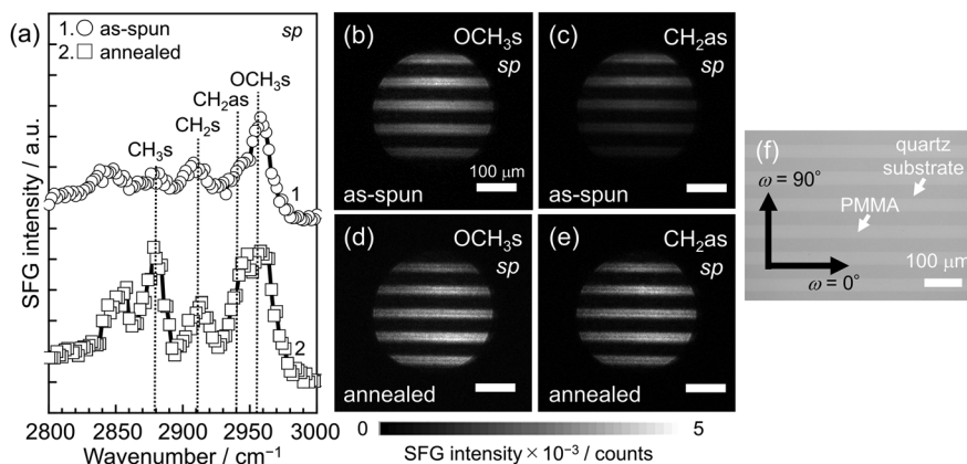
Fig. 2 (a) SFG spectra in the CH region with the sp polarization combination for a thin PMMA L&S film before (top) and after (bottom) annealing at 433 K for 24 h. SFG images for \text{OCH}_{3s} and \text{CH}_{2as} signals with the sp polarization combination for the (b and c) as-spun and (d and e) annealed films. (f) A digital microscopic image of the film. The angle formed with the line pattern ( \omega ) is shown.
